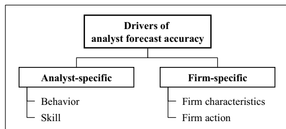
Figure 1: Drivers of analyst forecast accuracy
