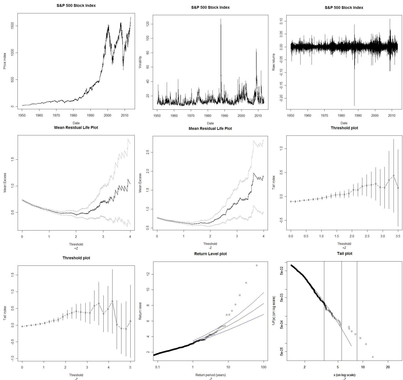
Figure 1. S&P 500 stock index. The Figure displays graphics from S&P 500 stock index from 3 January 1950 to 28 May 2013. From upper left to lower right corner: The stock index prices. The ARMA(1,1)-TGARCH historical volatility. The raw returns. The next four plots for visual threshold selections from the S&P 500 stock price standardized log-returns. ( +Z ) stands for upper tail and ( -Z ) stands for lower tail. The mean residual life plots are approximately linear with positively sloped, which indicates Pareto behavior overall for the -Z lower tail. The threshold plots display the maximum likelihood estimates for the tail index \xi against a range of thresholds with 95% confidence limits. The stability in the parameter estimates is checked when the parameter estimates are approximately constant above the threshold range. The last two plots display for the lower tail -Z , the 100-year return level for the fitted GPD with 95% confidence intervals and tail plot based on a generalized Pareto model fitted to losses over the -Z -threshold where the three vertical lines (from left to right) locate the 99%, 99.90% and 99.99% expected shortfall level.
