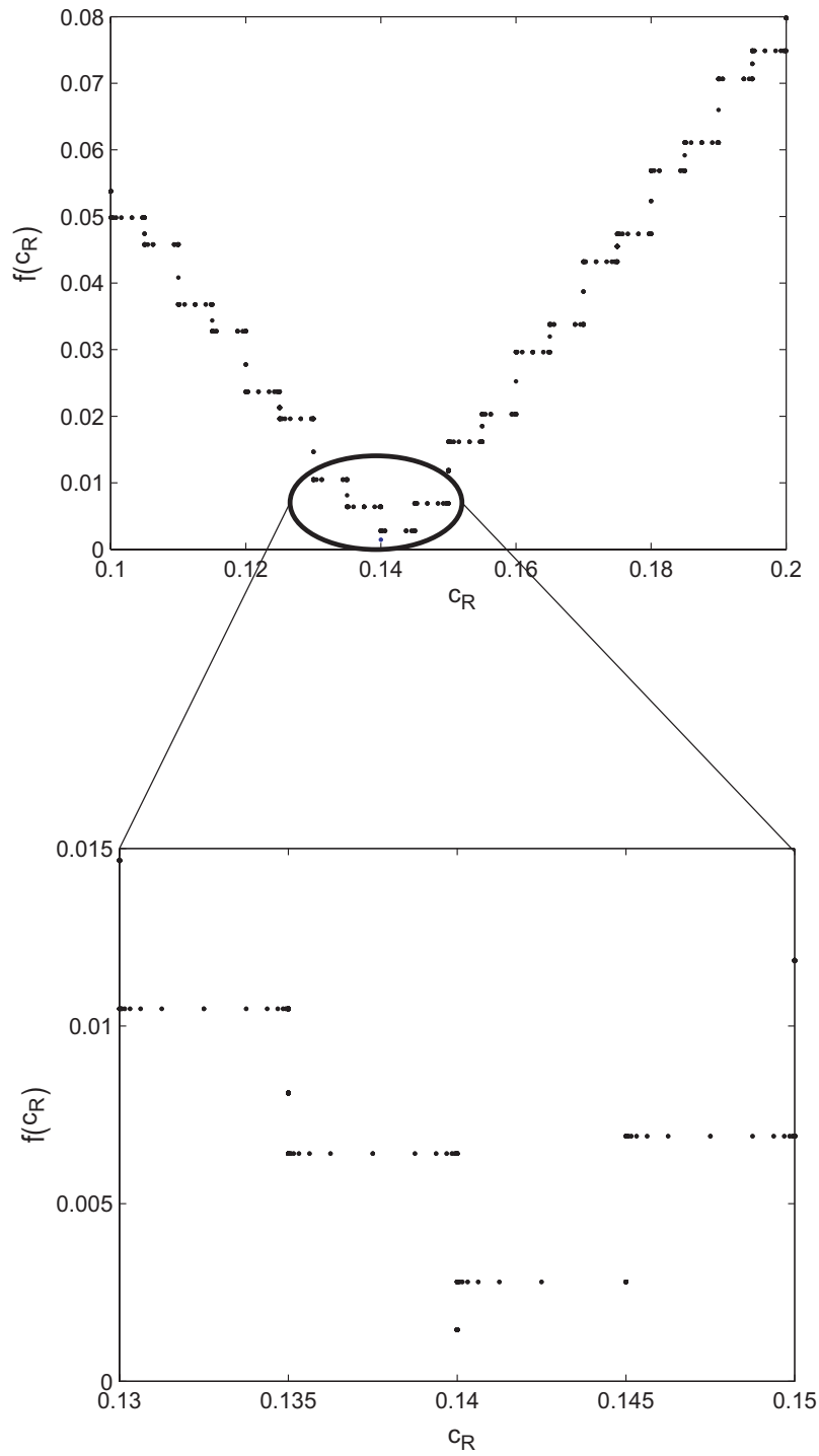
Figure 2. The objective function and zoom of the stop-loss reinsurance optimization problem.
