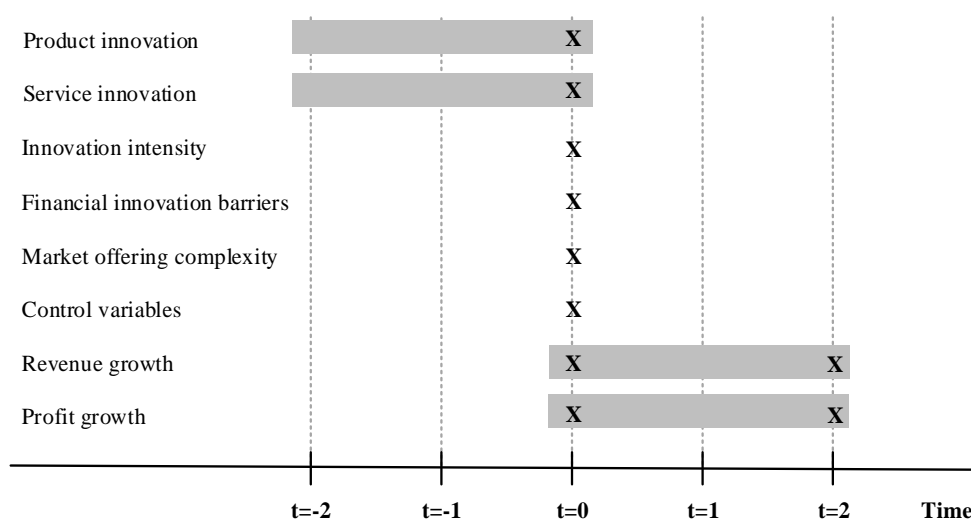
Fig. 2: Measurement waves and data points
