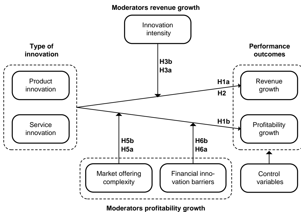
Fig. 1: Overview of the theoretical model
