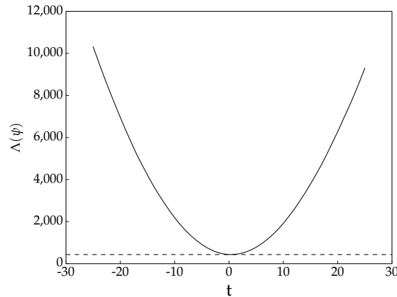
Figure 6: Criterion Function
