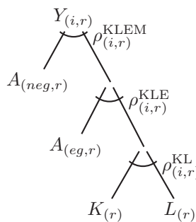
Figure 5: Structure of KLEM production function in Basic WIOD CGE Model
