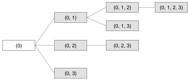
Figure 9: Exemplary decision tree
