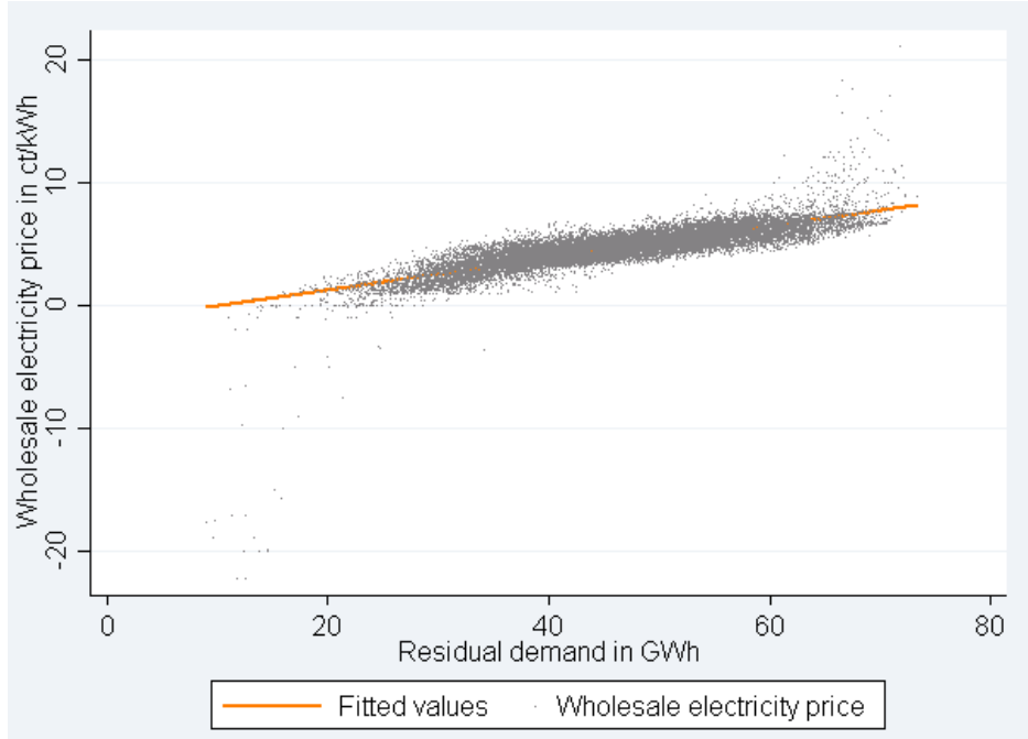
Figure 1: Scatter plot with linear regression line
