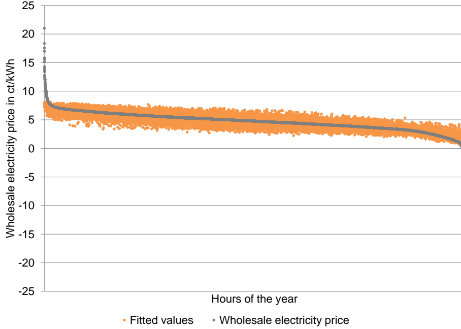
Figure 2: Annual price duration curves: Comparison of simulated and real wholesale prices in 2011 and 2012
