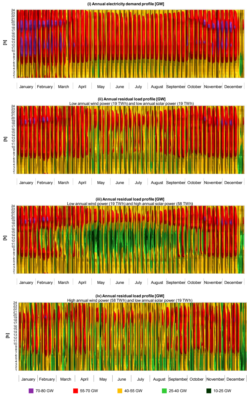
Figure A.7: Impact of increased wind and solar power penetration on the annual residual electricity demand profile (based on 8760 h)
