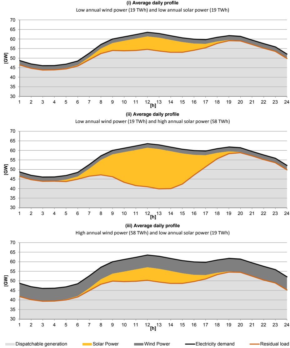
Figure 5: Impact of an increased wind and solar power penetration on the average daily residual load profile (based on 8760 h)
