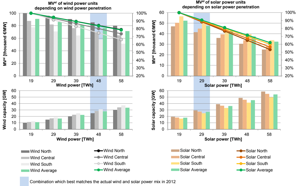
Figure 3: MV^{el} of wind and solar power units depending on their penetration level [€/MW]
