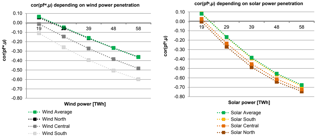
Figure 4: Correlation between the hourly wind/solar power production factor and the wholesale price
