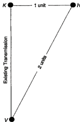
Figure 1: Coordination problem in generation and transmission expansion (Baldick and Kahn 1993, p. 373)
