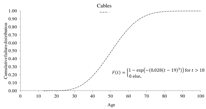
Figure 5: Cumulative failure distribution of medium voltage cable
