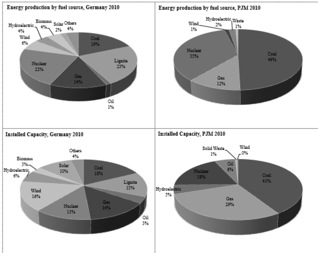
Figure 1: Comparison of generation indicators for PJM and Germany (2010)
