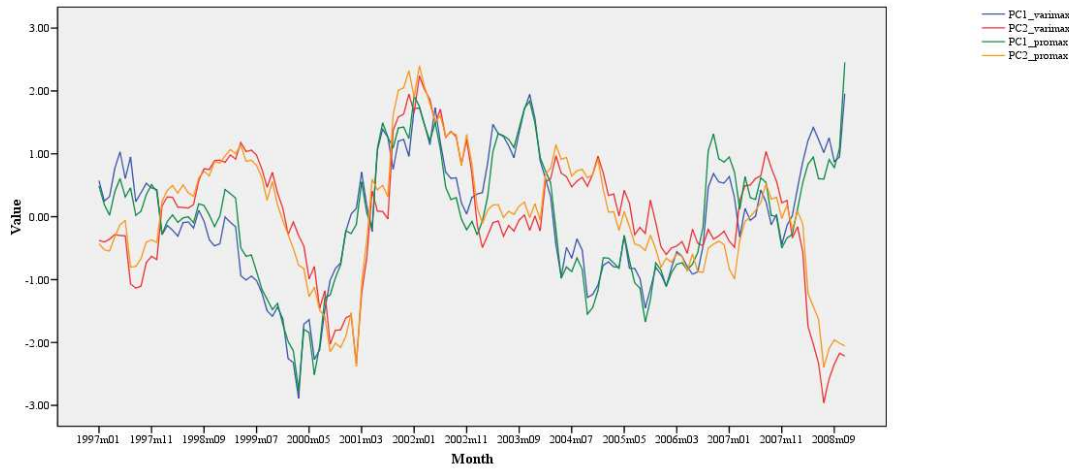
Figure 10: First and second PCs, 370 \Delta_{i,j}^{HH_{\text{specific}}} series, 1997m01-2008m11 ( n = 143 ), varimax and promax rotated
