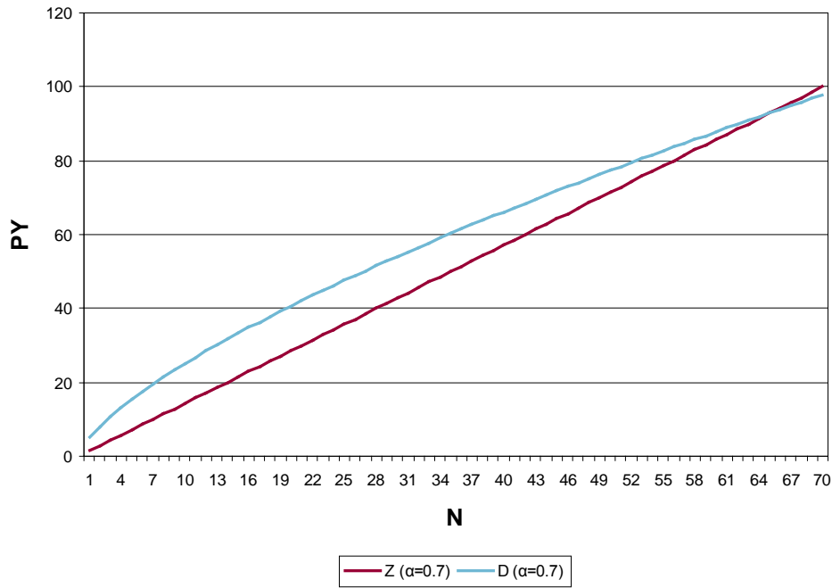
Figure 2: Simulated D and Z functions for Y(N)=N^{0.7}
