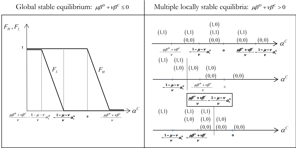
Figure 2: set of equilibria, (F_H, F_L) for the right column.
