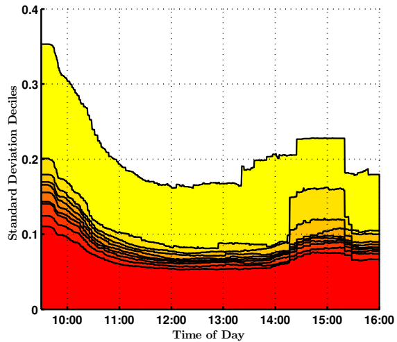
(b) Volatilities
