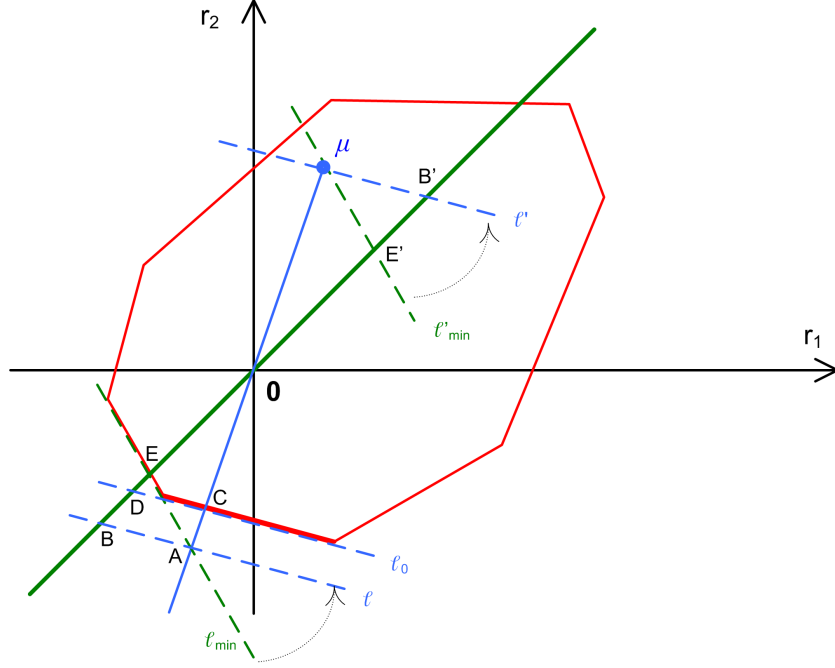
Figure 2: Searching the Sharpe ratio optimized portfolio.
