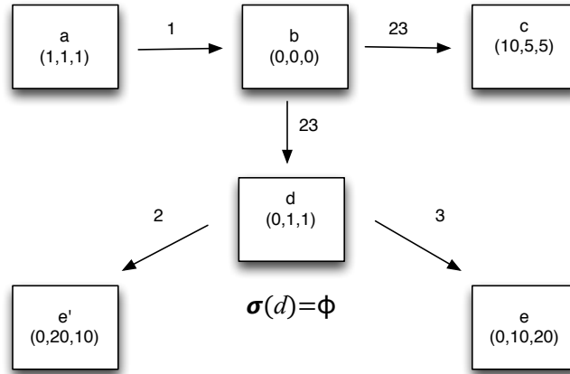
FIGURE 6. ILLUSTRATION OF EXAMPLE 10.
