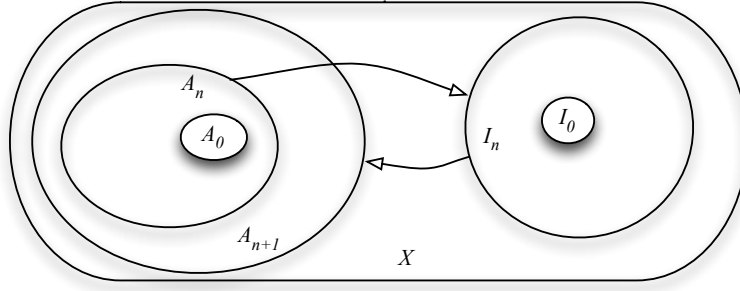
FIGURE 3. RECURSIVE DEFINITION FOR CREDIBILITY OF FAR-SIGHTED OBJECTIONS
