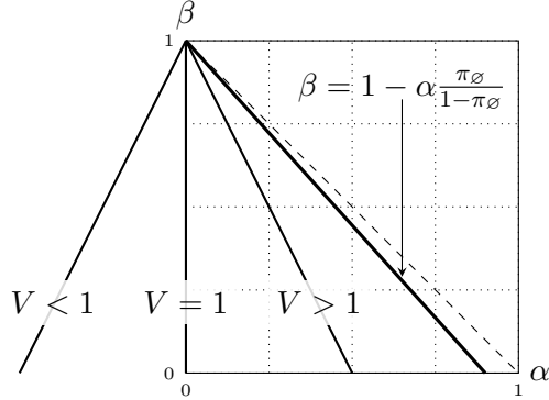
Figure 1: The shape of the zero-surplus curve for \pi_\emptyset \geq \frac{1}{2}
