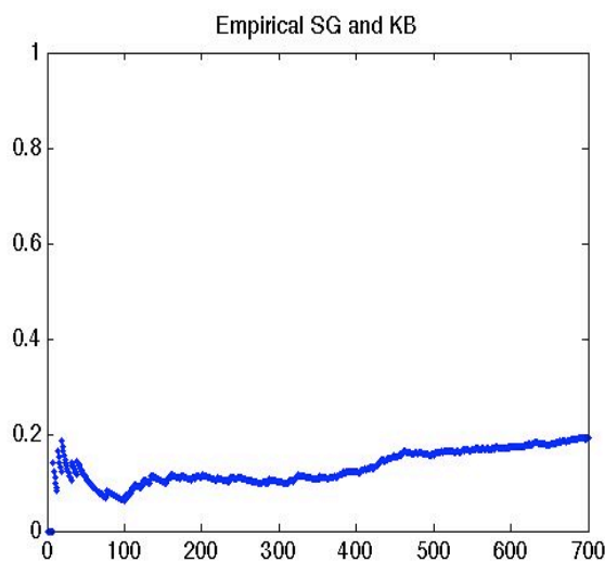
Figure 3: Conditional number of failures (minus one) estimated from the returns of SG and KB.
