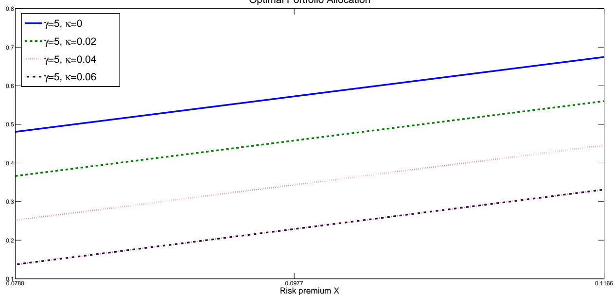
Figure 4: Optimal Portfolio Allocation
