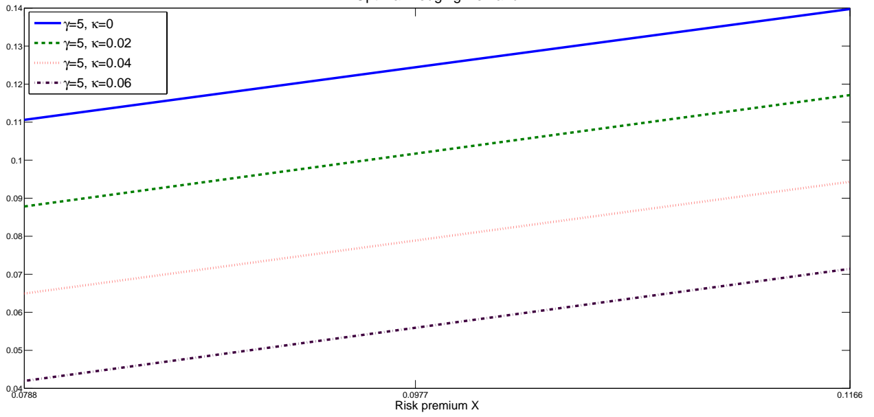
Figure 3: Optimal Hedging Demand
