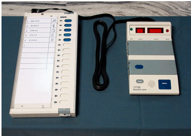
Figure 2: Indian EVM consisting of a ballot unit (left) and a control unit (right) joined by a five-meter cable. (Prasad et al, 2010).
