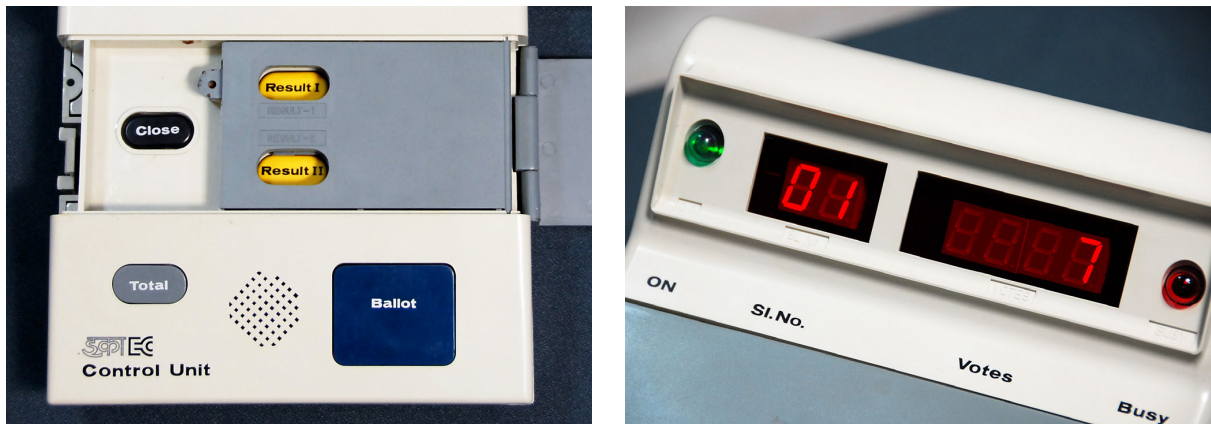
Figure 3: Behind plastic doors there is black close button and result button (left). Display unit on the right (Prasad et al, 2010).
