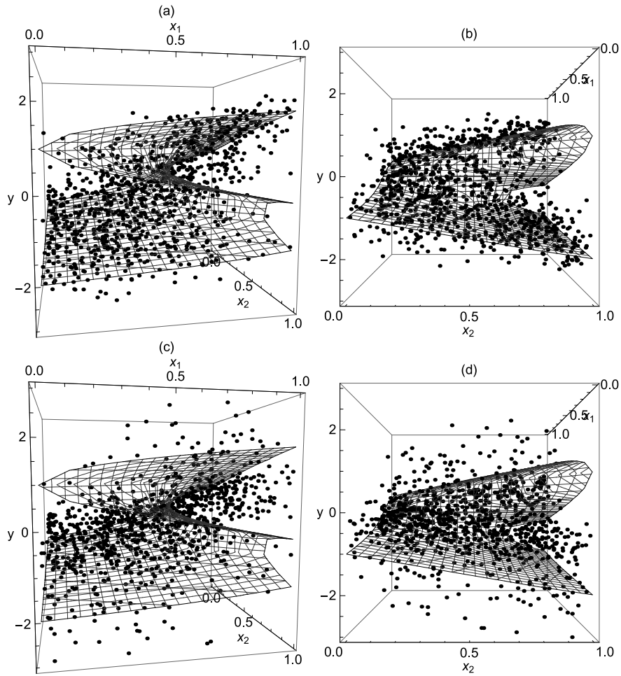
Figure 2: An example of simulated data where the cusp surface is subject to noise only, y_t , and noise with volatility, r_t . Parts (a-b) show the cusp deterministic pleat simulated \{x_1, x_2, y_t\} from two different perspectives, and parts (c-d) show the cusp deterministic pleat simulated \{x_1, x_2, r_t\} from two different perspectives.
