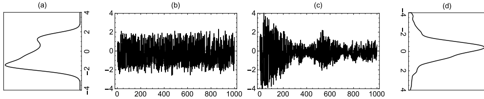
Figure 1: An example of a simulated time series where the cusp surface is subject to noise only, y_t , and noise together with volatility, r_t . (b) simulated returns y_t (a) kernel density estimate of y_t (c) simulated returns r_t contaminated with volatility (d) kernel density estimate of r_t .
