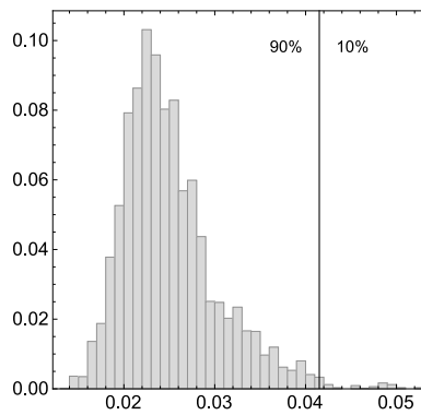
Figure 6: Histogram of the dip statistics for bimodality computed for all of the rolling window periods, together with the bootstrapped critical value 0.0406 for the 90% significance level plotted in bold black.
