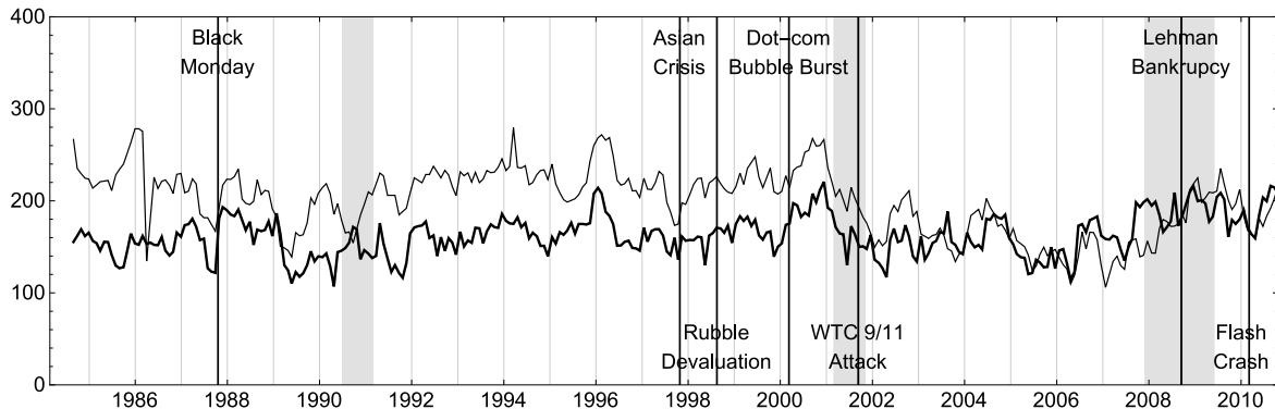
Figure 5: Rolling values of BIC information criteria for the cusp catastrophe (in bold black) and the logistic (in black) models.
