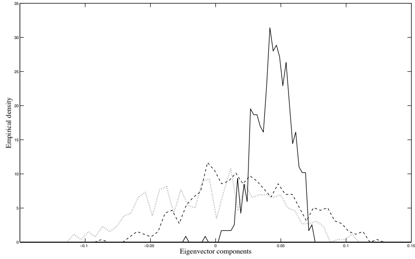
Figure 1. Empirical component distributions of the top correlation matrix eigenvectors for financial returns (solid line), profit rates (dashed), and synthetic returns from equation (5)
