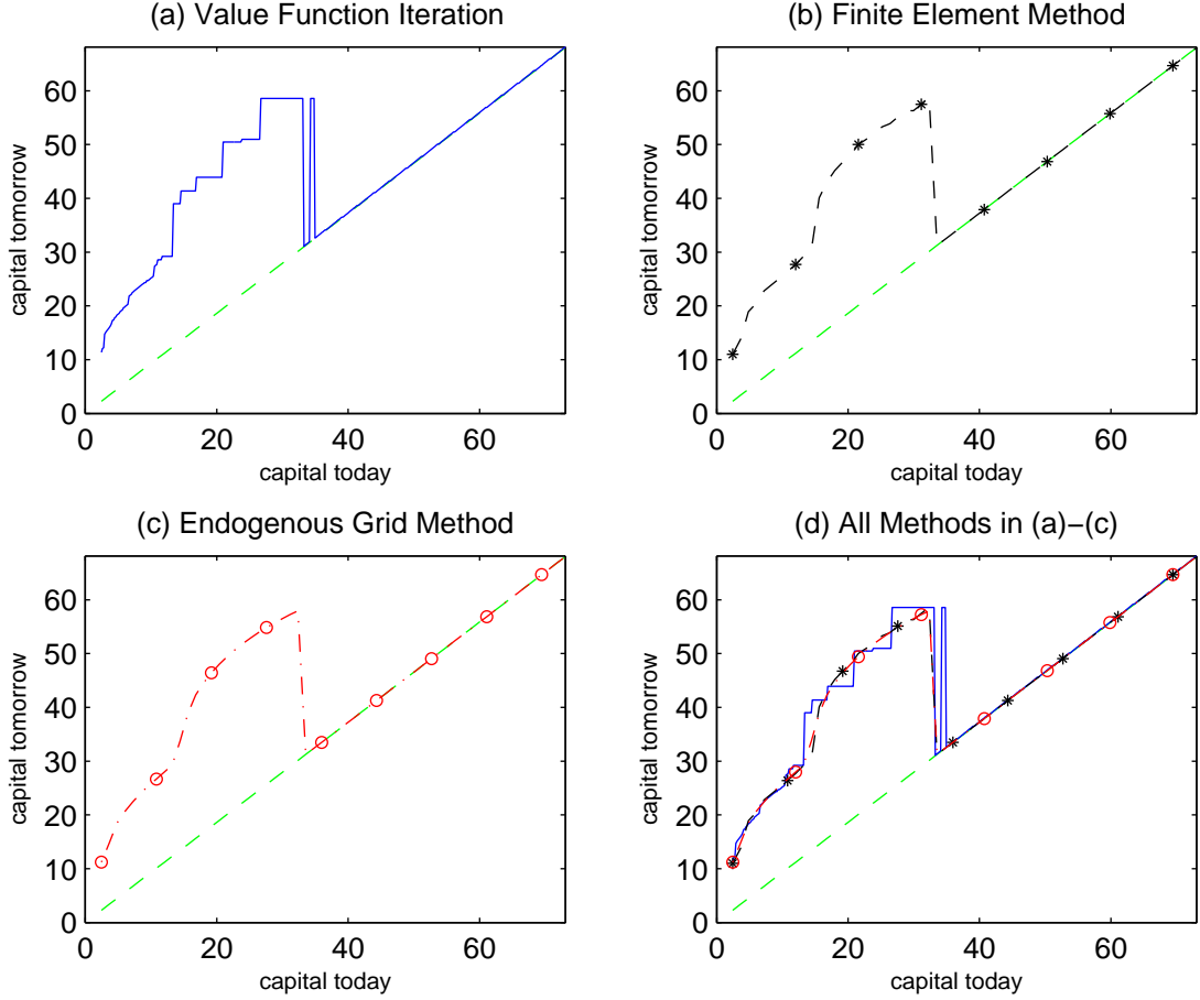
Figure 2: Policy Function for capital (given A = e^{0.0372} ) implied by different approximation methods. The green dashed line indicates the no investment decision (1 - \delta)K . The baseline capital grid (VFI: 420, FEM: 60, EGM: 60) generates comparable average log-absolute Euler equation errors across methods.
