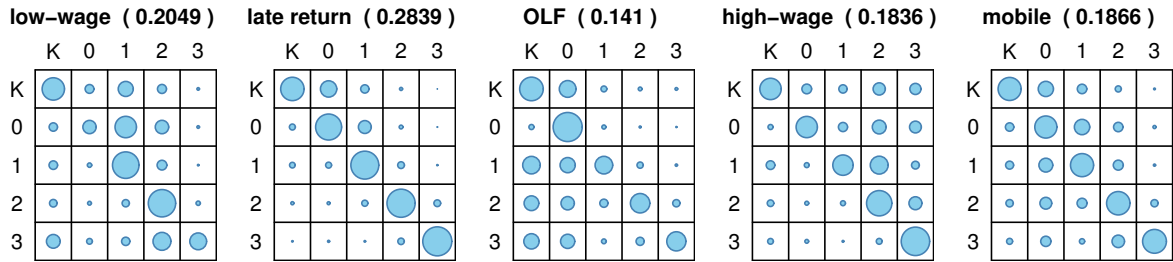
Figure 2: Visualization of posterior expectation of the transition matrices \xi_1, \xi_2, \xi_3, \xi_4 , and \xi_5 obtained by Markov chain clustering. The circular areas are proportional to the size of the corresponding entry in the transition matrix. The corresponding group sizes are calculated based on the posterior classification probabilities and are indicated in the parenthesis. K=parental leave, 0=out of labor force, 1=low wage employment, 2=middle wage, 3=high wage.
