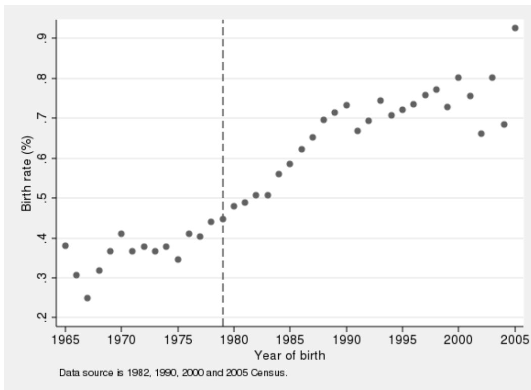
Figure 1 Twins Rates Against Year of Birth
