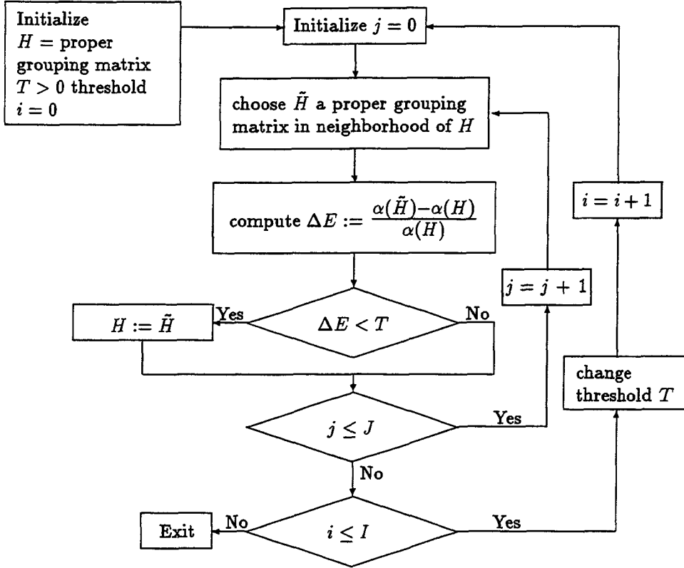
Figure 2: Threshold Accepting Algorithm for Optimal Aggregation
