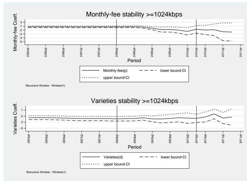
Figure 5: Structural stability of demand parameter estimates
