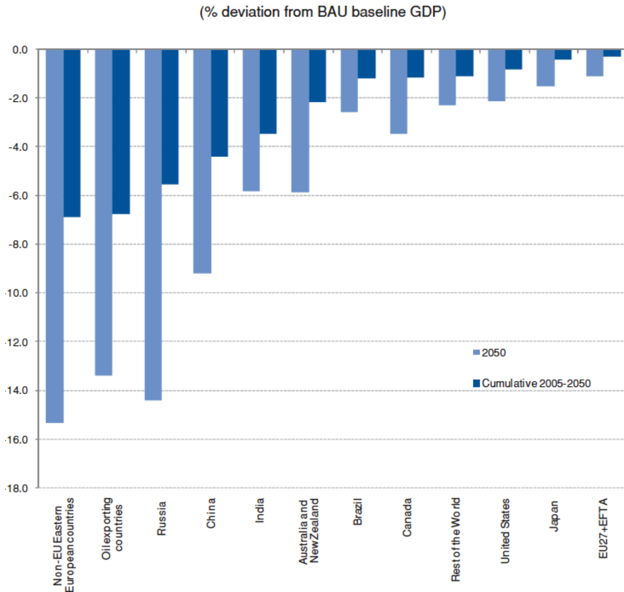
Figure 6: Costs from Stabilizing Long-Run GHG Concentration at 550 ppm Across Regions
