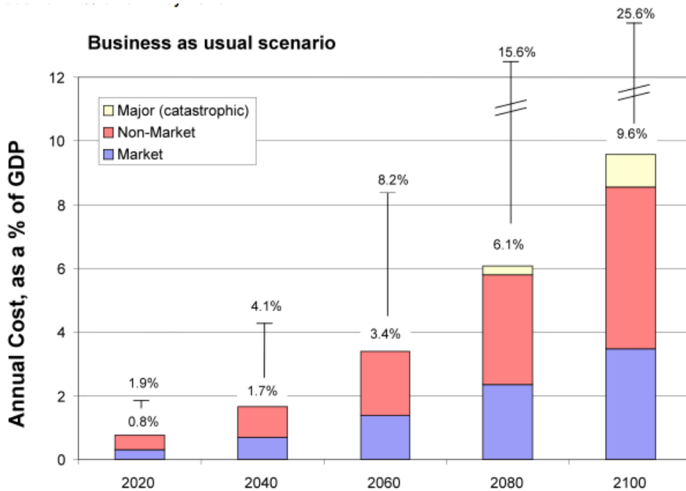
Figure 2: Equivalent Annual Cost of Climate Change in Africa, as a % of GDP
