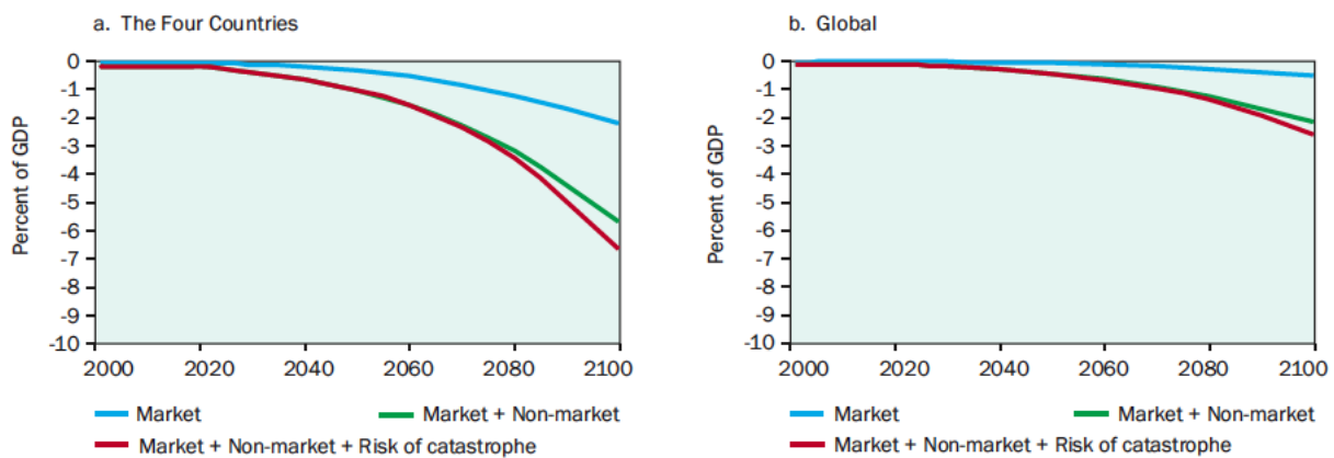
Figure 3: Mean Impact of Climate Change on Southeast Asian Countries and at the Global Scale, as a % of GDP
