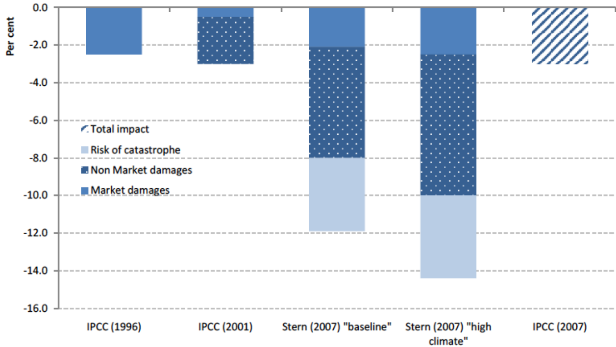
Figure 1: Estimates of the Global Damages of Climate Change (% of world GDP)
