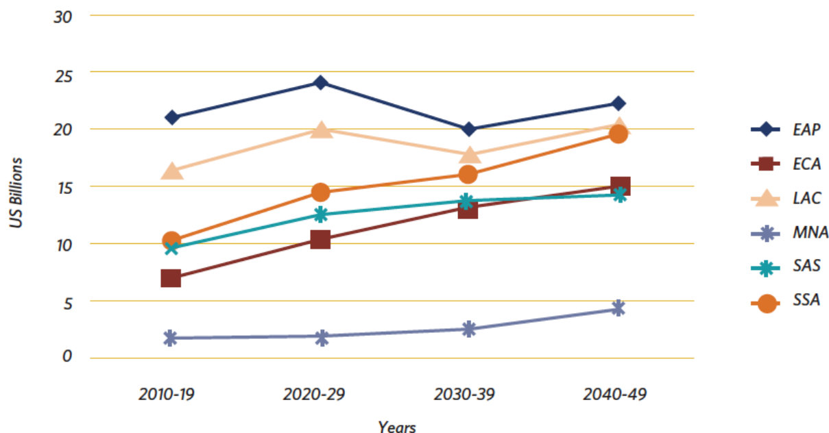
Figure 5: Total Annual Cost of Adaptation for the NCAR Scenario, by Region and Decade (US$ billions at 2005 prices, no discounting)
