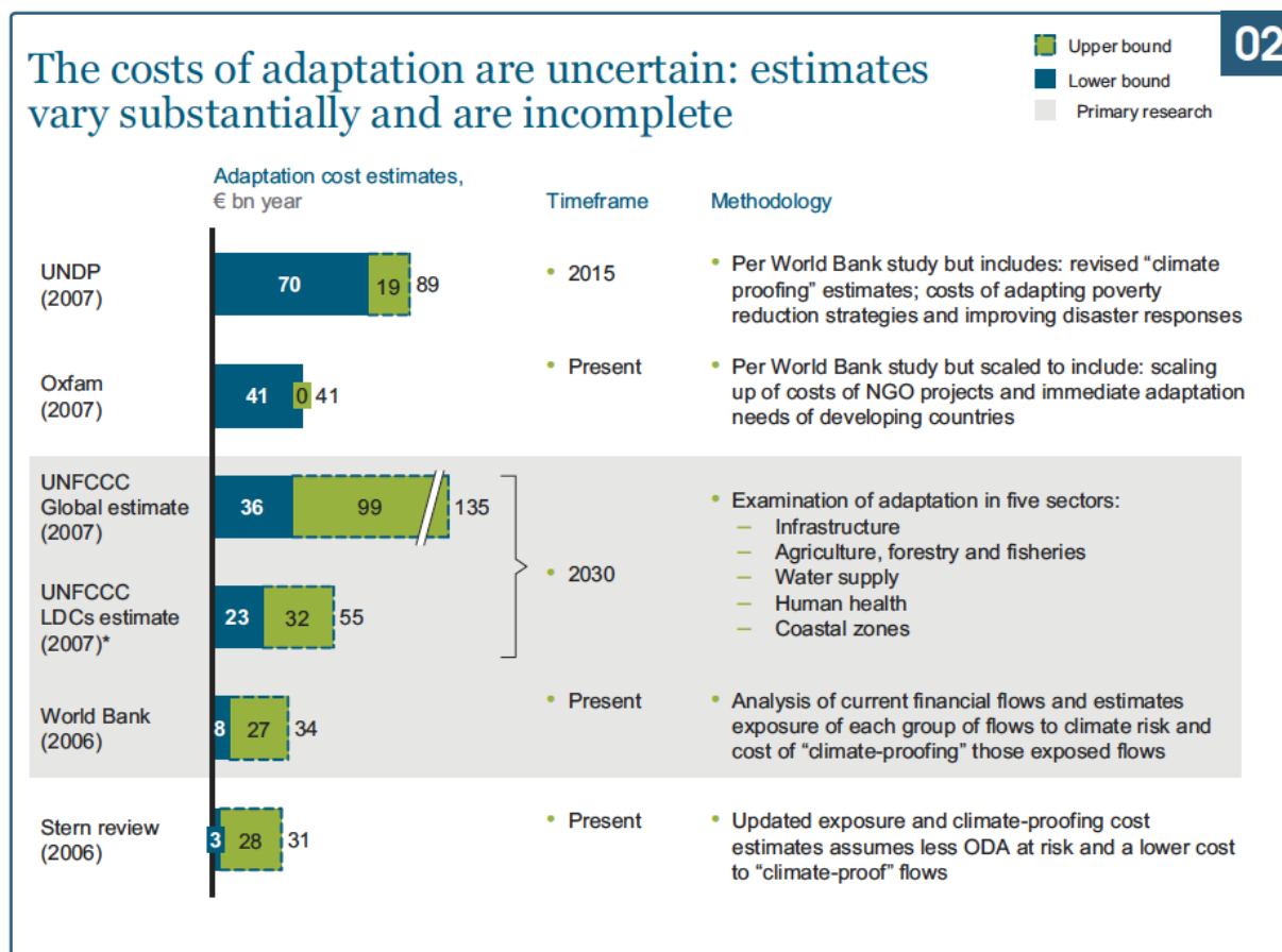
Figure 4: Adaptation Cost Estimates Based on Various Methodologies
