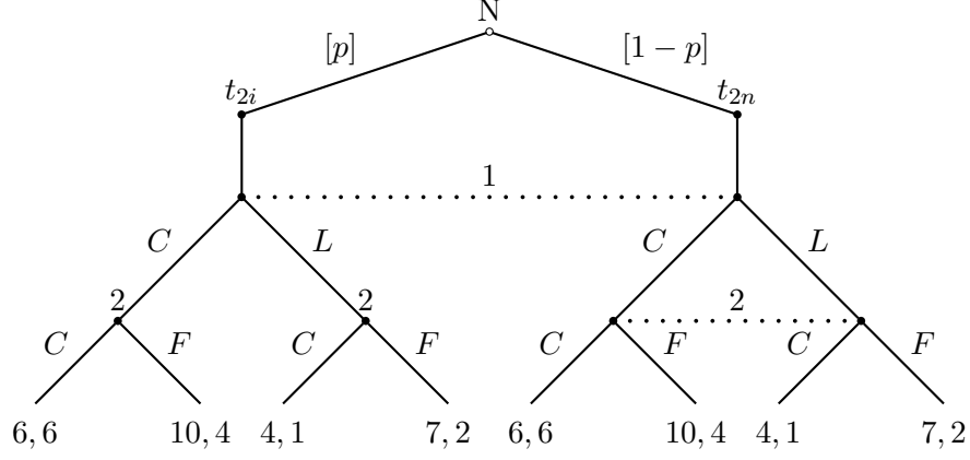
Figure 2: Meta Game
