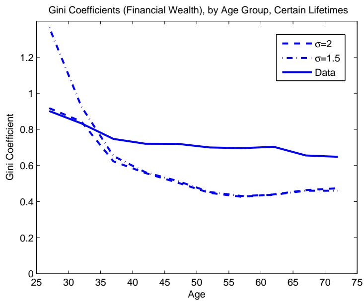
Figure 3: Gini Coefficients: Non-Housing Assets
