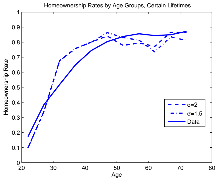
Figure 2: Homeownership Rates by Age Group
