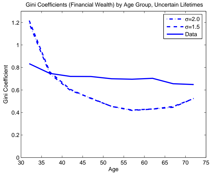
Figure 5: Gini Coefficients: Non-Housing Assets
