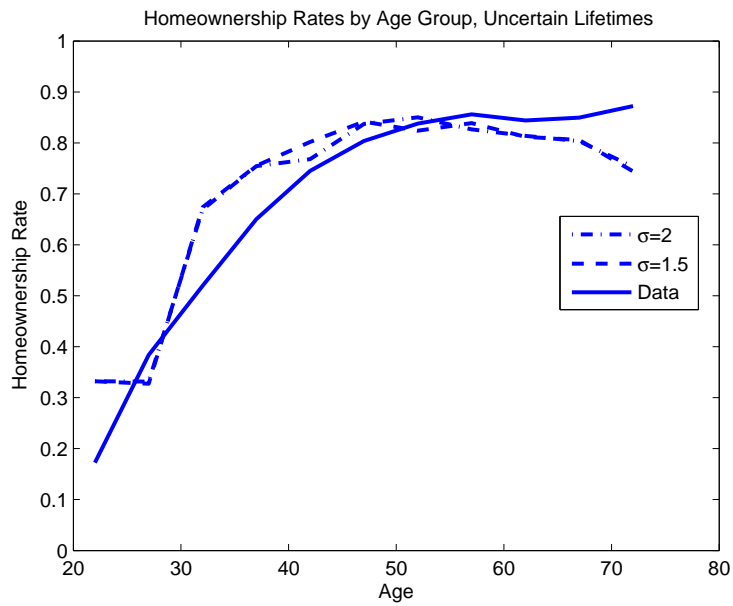
Figure 7: Homeownership Rates by Age Group
