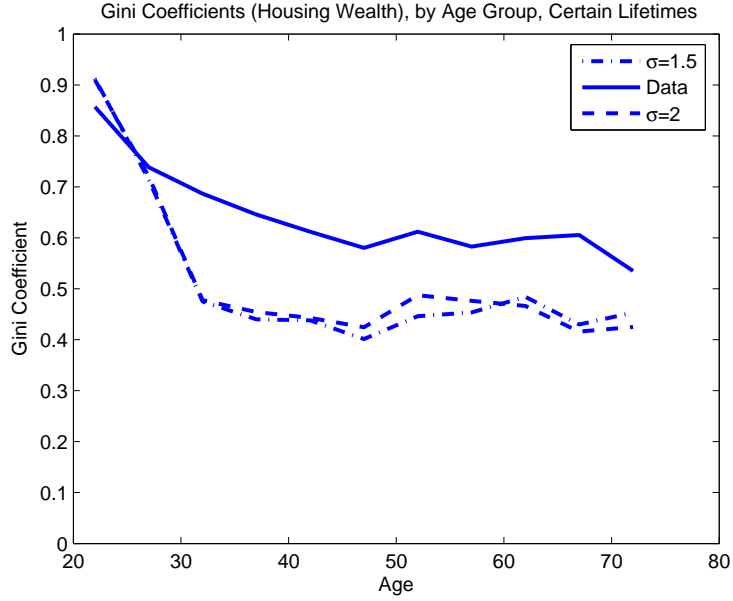
Figure 4: Gini Coefficients: Primary Residence
