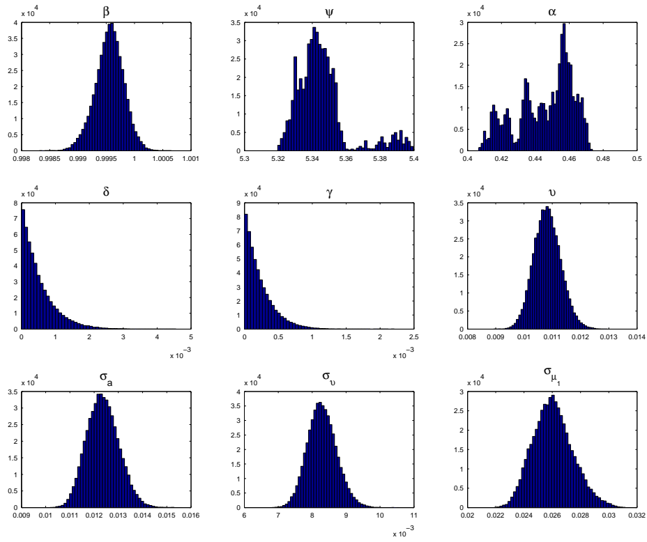
FIGURE 2. Posterior distribution for the structural parameters of Fisher's model.
