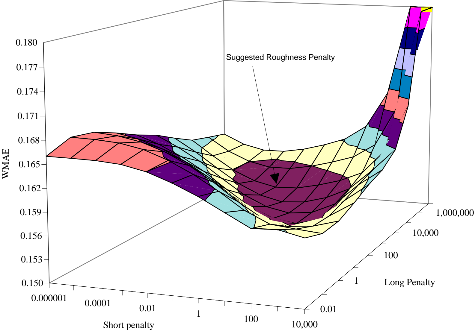
Figure 5: Out-of-sample weighted mean absolute error of securities between 1 and 10 years to maturity
