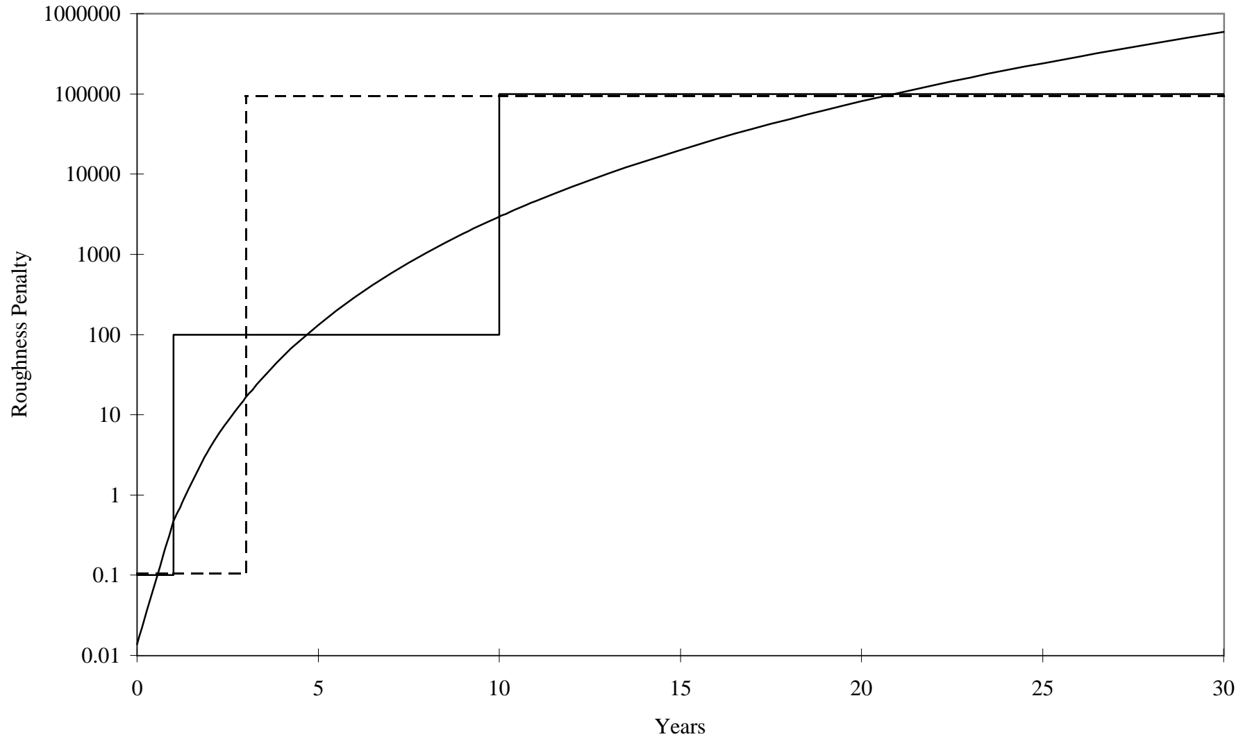
Figure 3: Sample Roughness Penalty Shapes
