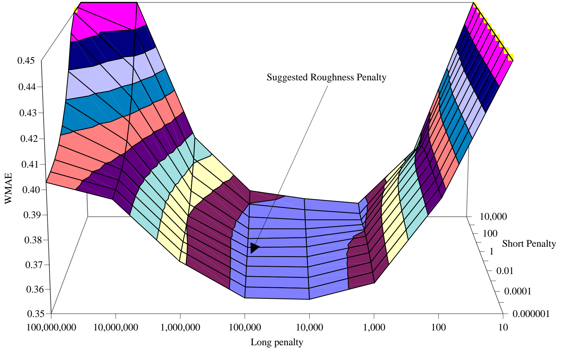
Figure 6: Out-of-sample weighted mean absolute error of securities with more than 10 years to maturity
