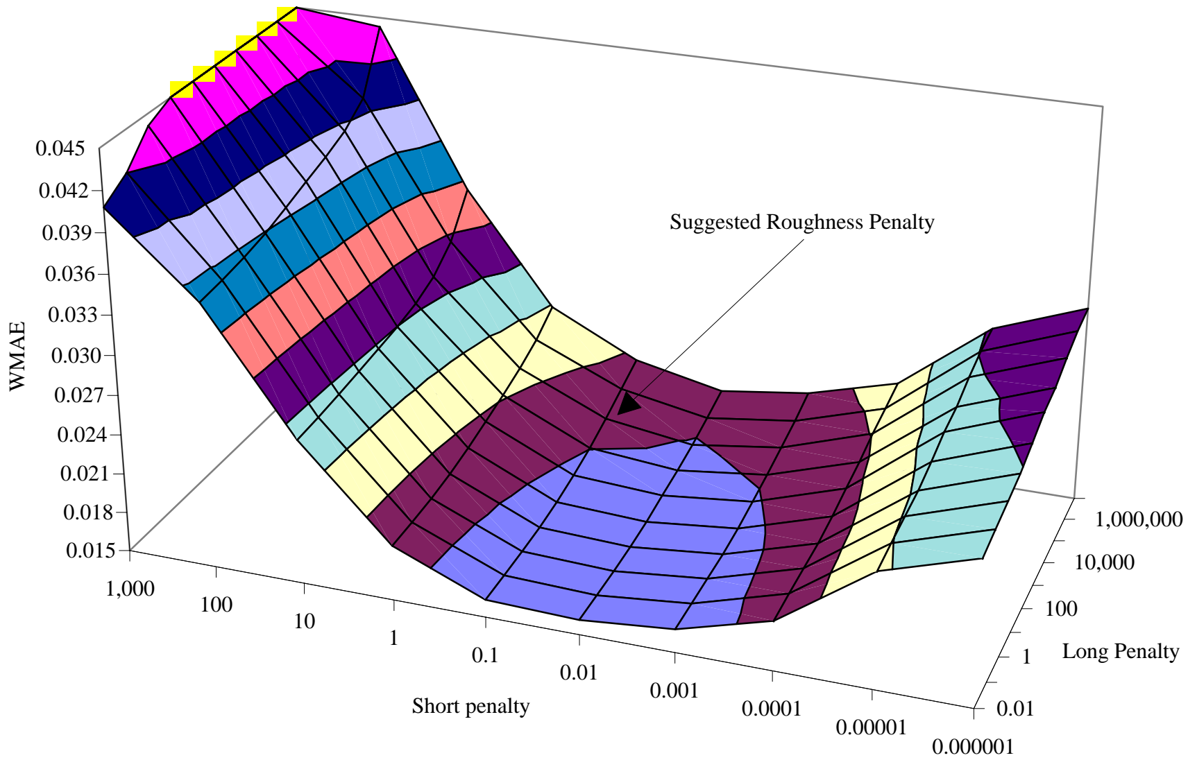
Figure 4: Out-of-sample weighted mean absolute error of securities with less than 1 year to maturity
