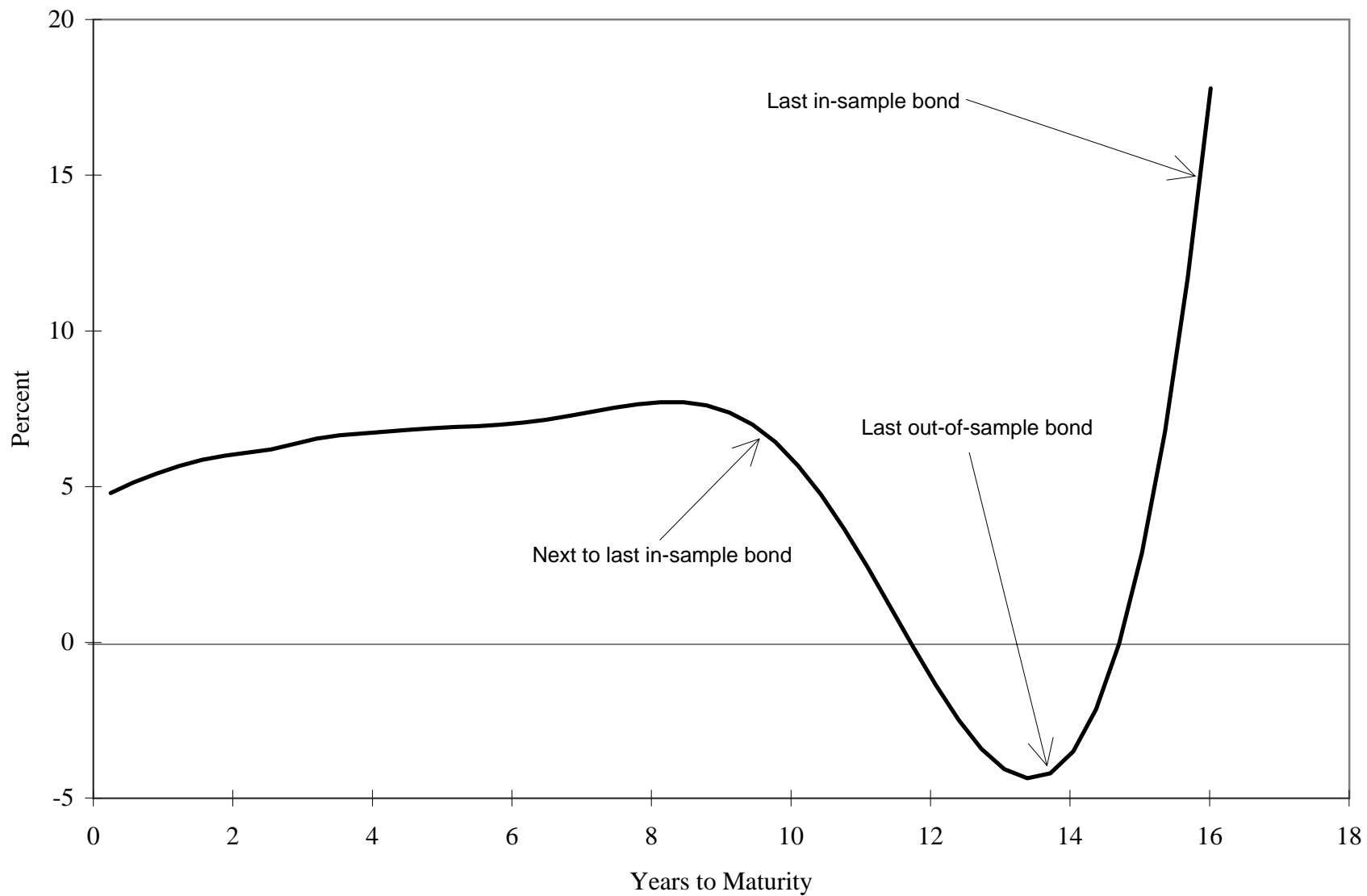
Figure 7: Fisher Yield Curve for February 28, 1977
