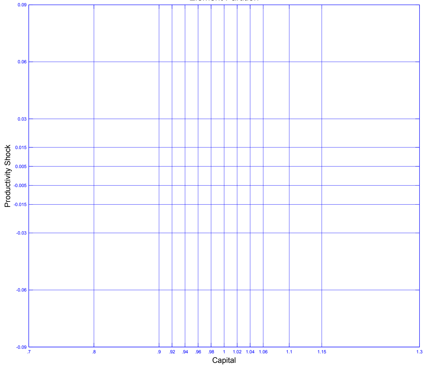
Figure A1: Finete Element Partition
