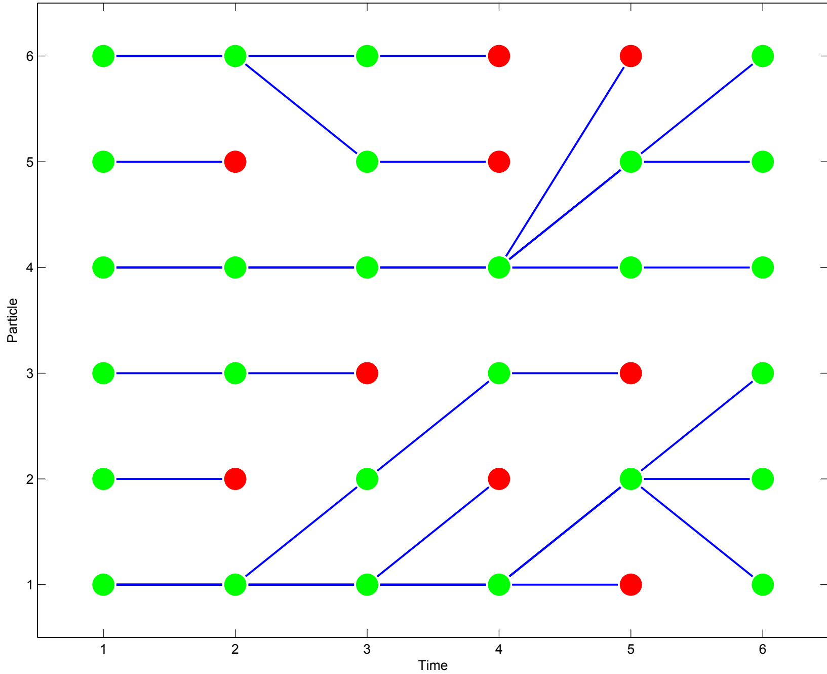
Figure 2.1: Particles evolving over time
