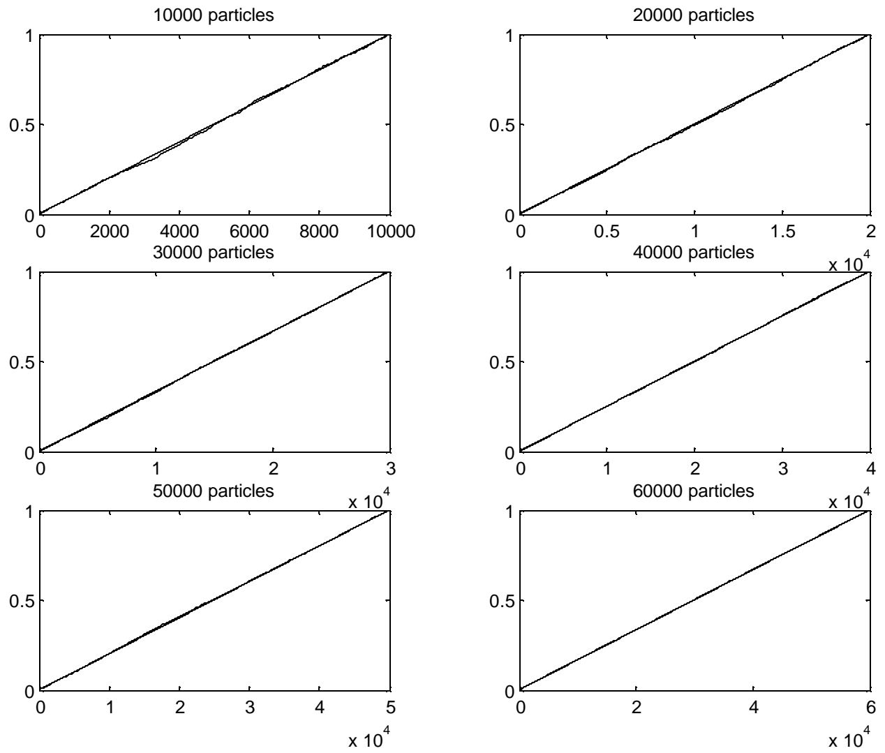
Figure 3.6: CDF Extreme Calibration
