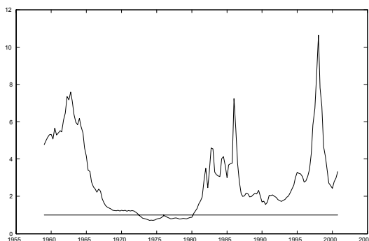
Figure 10: Estimates of the Activism Coefficient
