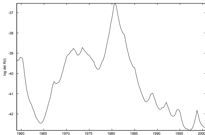
Figure 2: Total Prediction Variance
