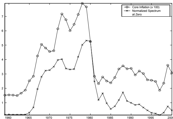
Figure 9: Core Inflation and Inflation Persistence
