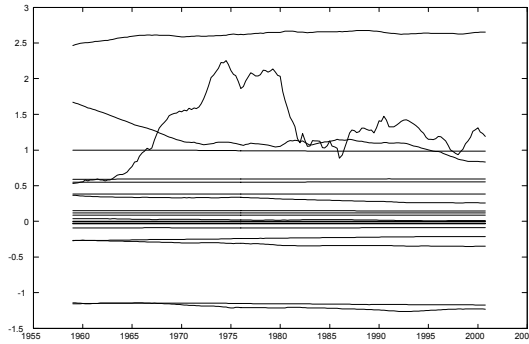
Figure 14: Principal Components of \theta_{t|T}
