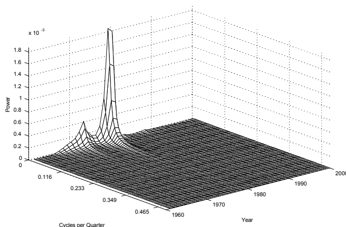
Figure 6: Spectrum for Inflation
