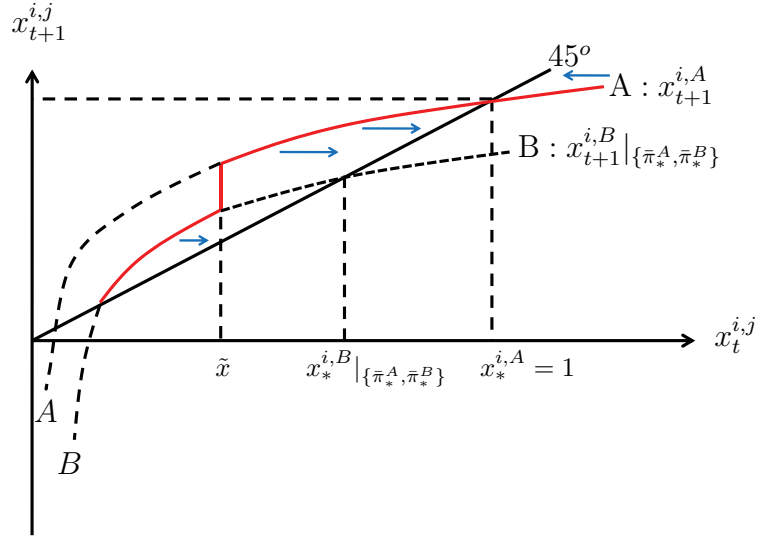
Figure 2: Evolution of relative human capital x_t^i . AA -locus: evolution of x_t^{i,A} . BB -locus: evolution of x_t^{i,B} given \{\bar{\pi}_t^A, \bar{\pi}_t^B\} .
