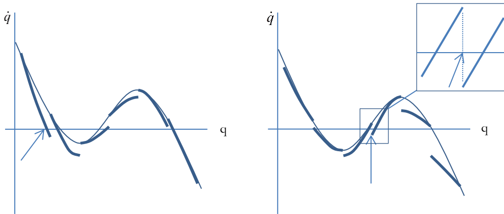
Figure 4: Effects of discontinuity on \dot{q}(q) . Left: \Delta^e > 0 , right \Delta^e < 0 :
