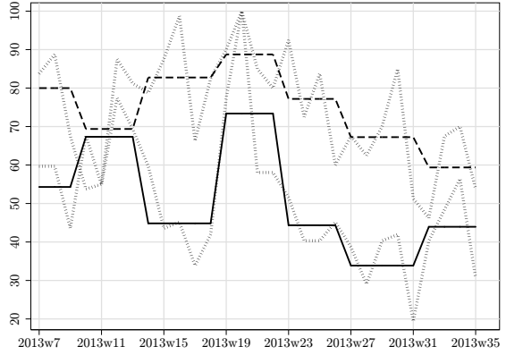
Figure 2: Unblocking YouTube
