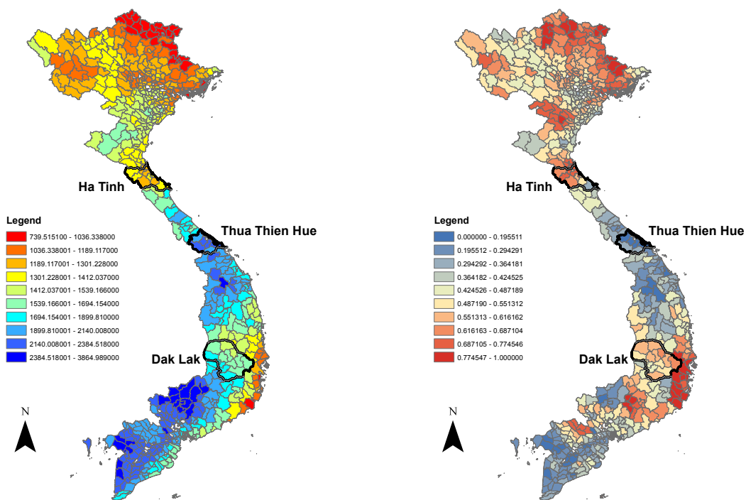
(a) Precipitation (mm) (b) Drought severity, 3-months average (mm)
