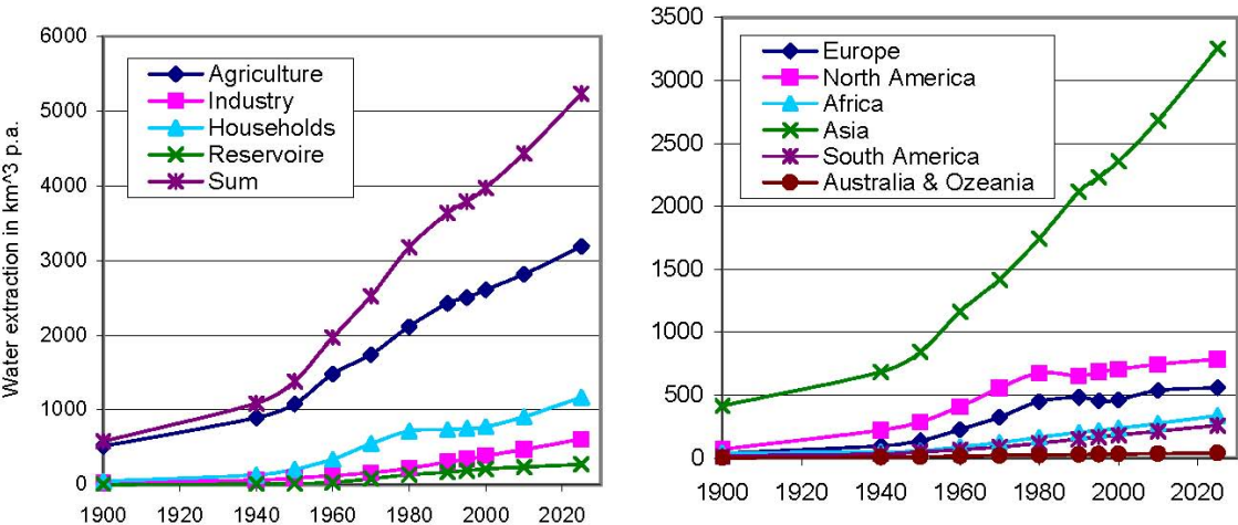
Fig. 3.2.10-1: Water withdrawal in different sectors and world regions (Source: Shiklomanov & Rodda 2003).
