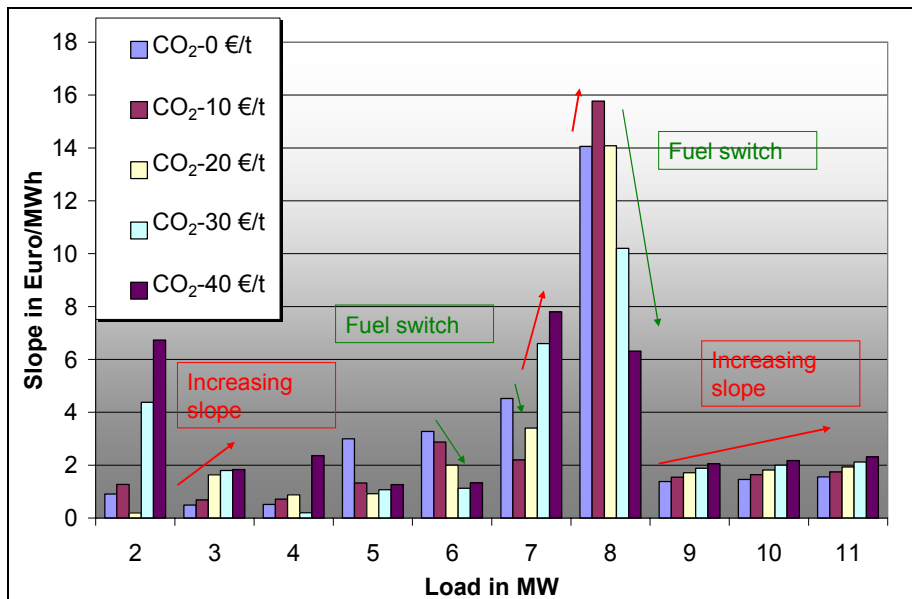
Figure 6: Slope of the merit-order curve
