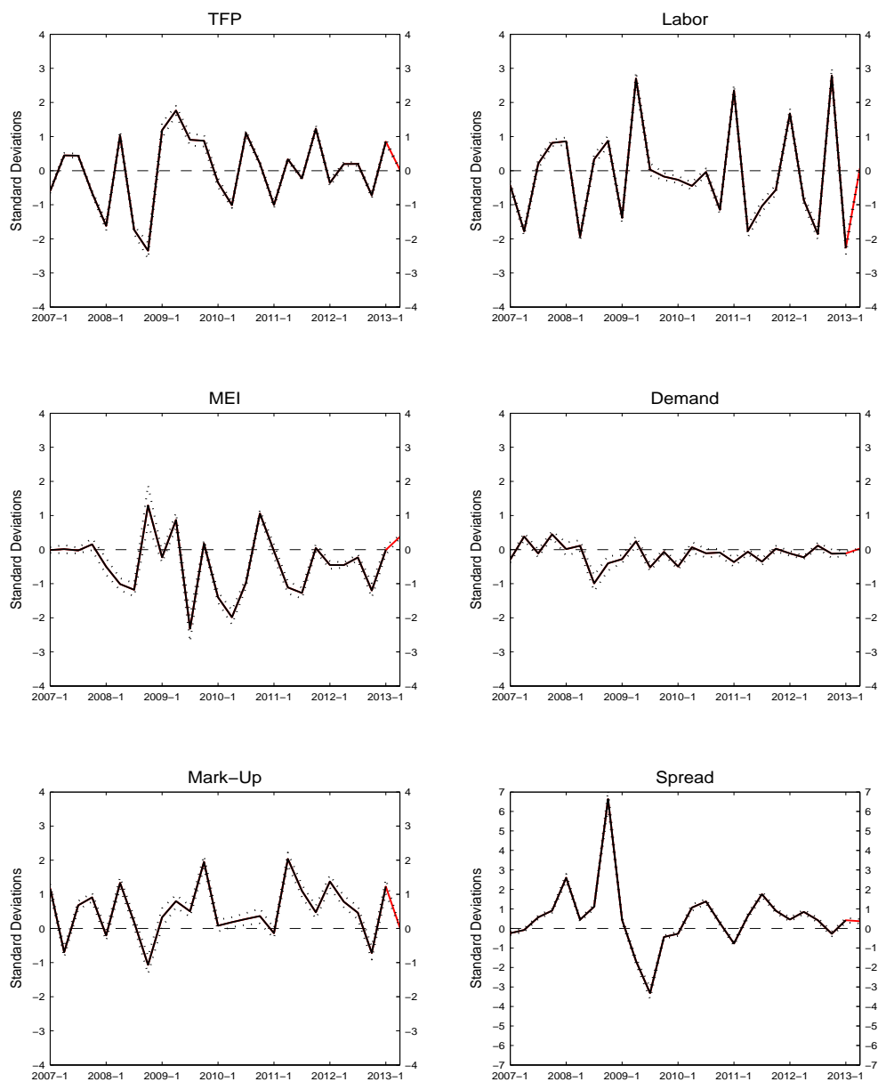
Figure 14: Shock Histories
