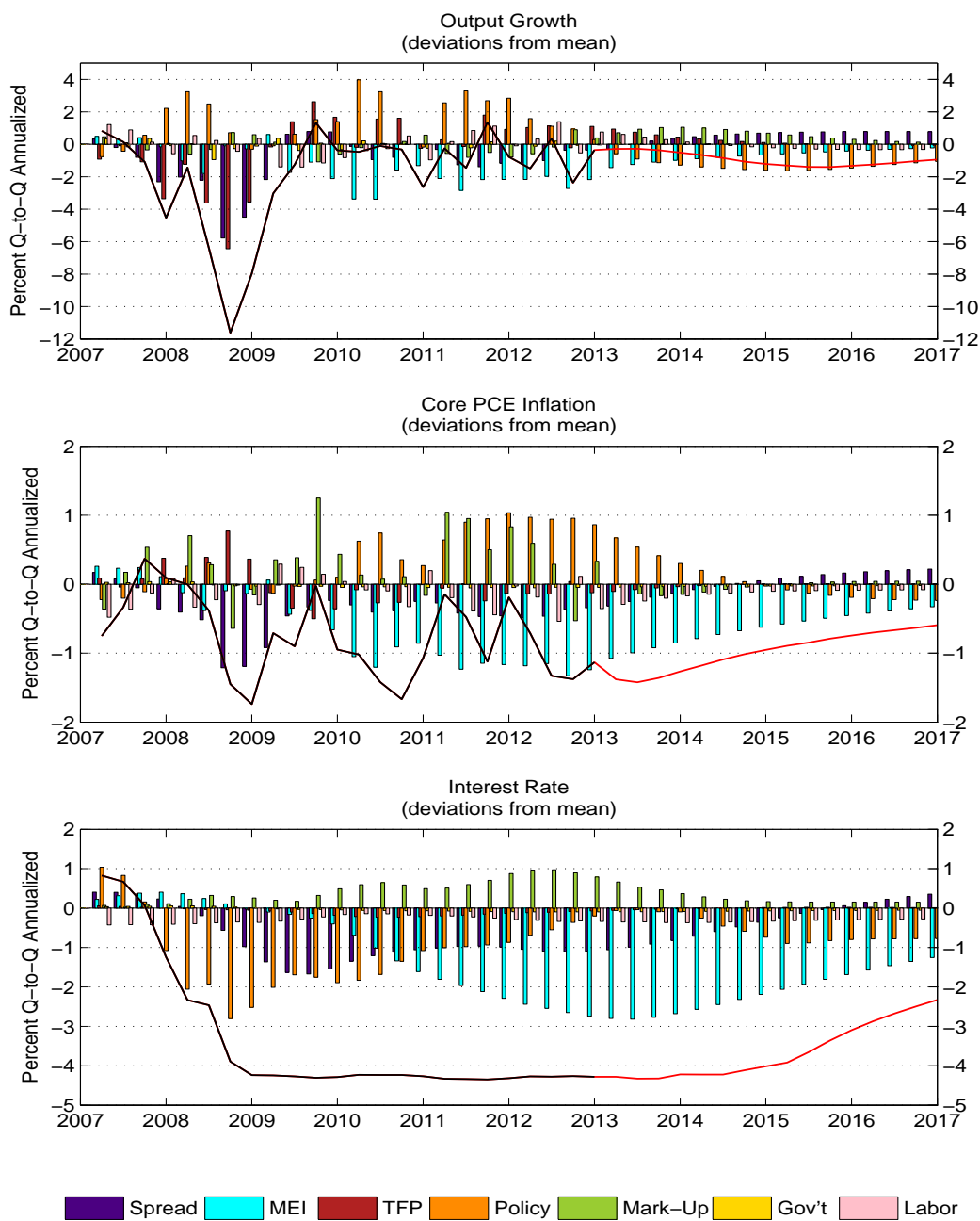
Figure 12: Shock Decomposition
