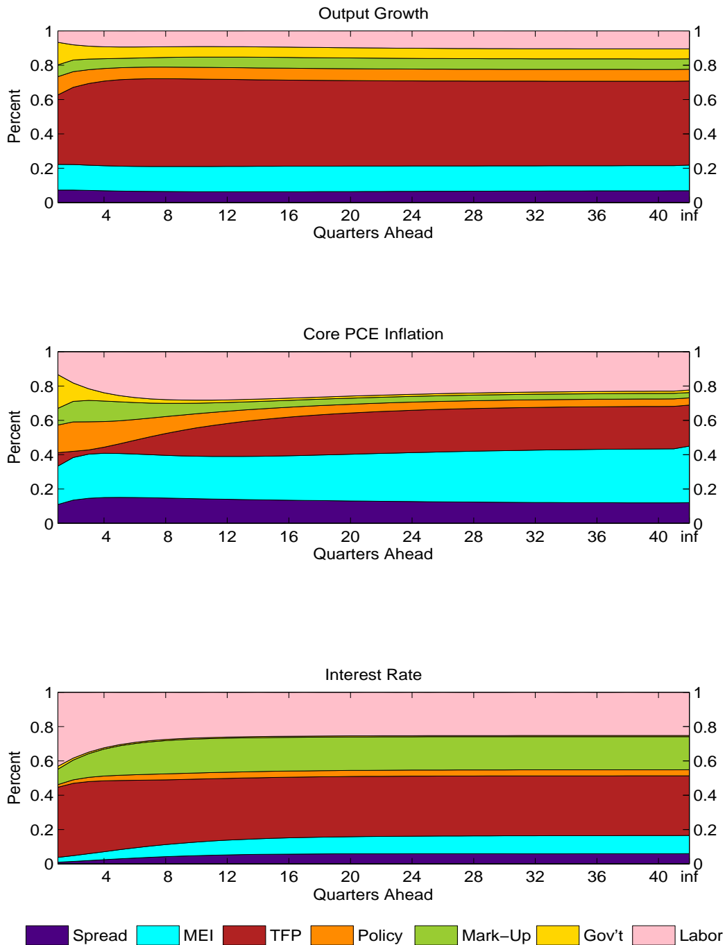
Figure 11: Variance Decomposition
