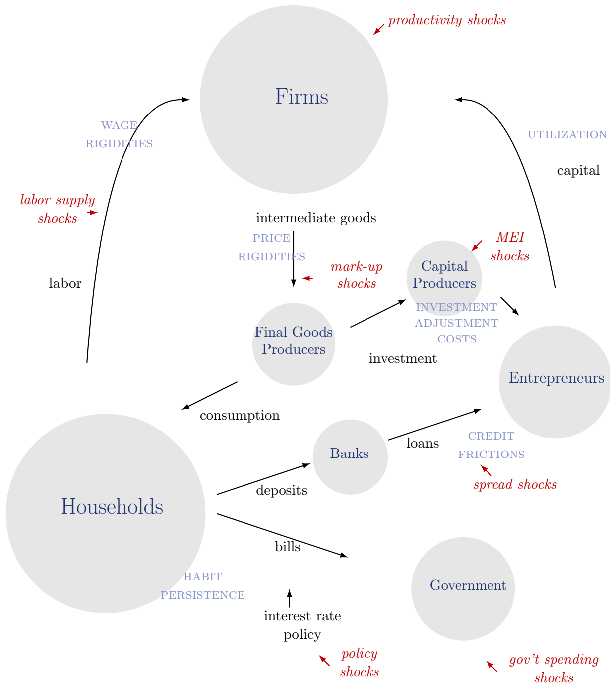
Figure 1: Model Structure
