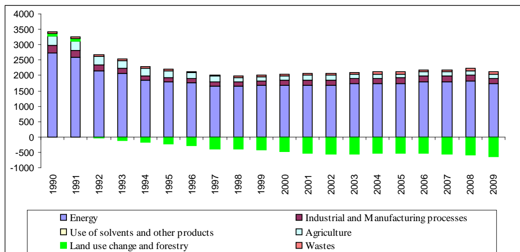
Figure 38. GHG Emissions (CO 2 , CH 4 , N 2 O, PFCs, HFCs, SF 6 ) in Russia by Sector (mln. tons CO 2 -eq)
