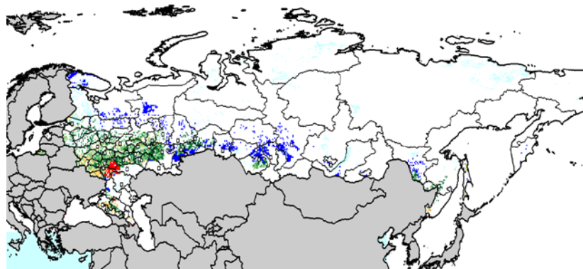
ECHAM5 GCM
