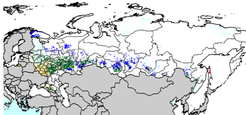
MIROC3.2 medium resolution GCM
