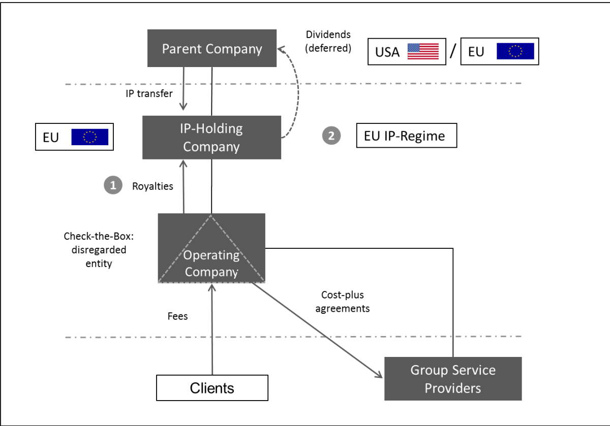
Figure 2: IP-Holding structure
