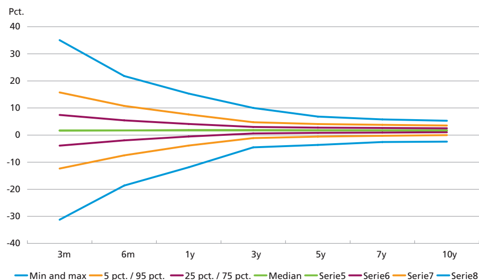
DISTRIBUTION OF RETURNS AT DIFFERENT HORIZONS Chart 21
