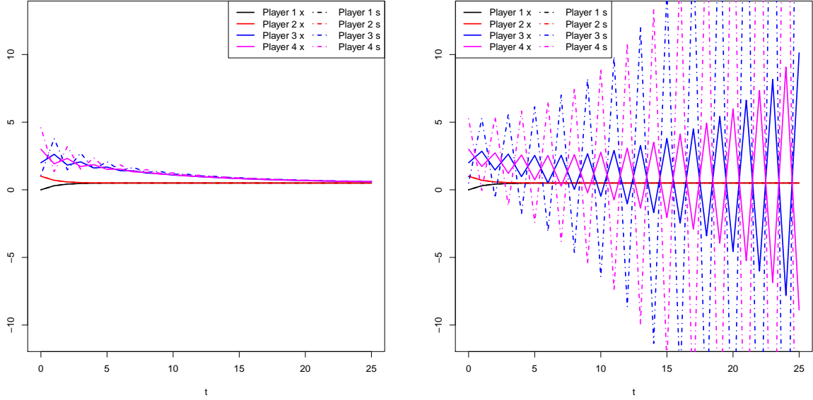
Figure 4: The opinion dynamics of Example 2 for (a) \delta_{\text{ROTW}} = -.75 and (b) \delta_{\text{ROTW}} = -.9 .
