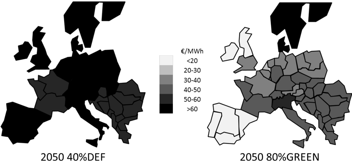
Figure 4: Peak load price levels in 2050, 40%DEF and 80%GREEN
