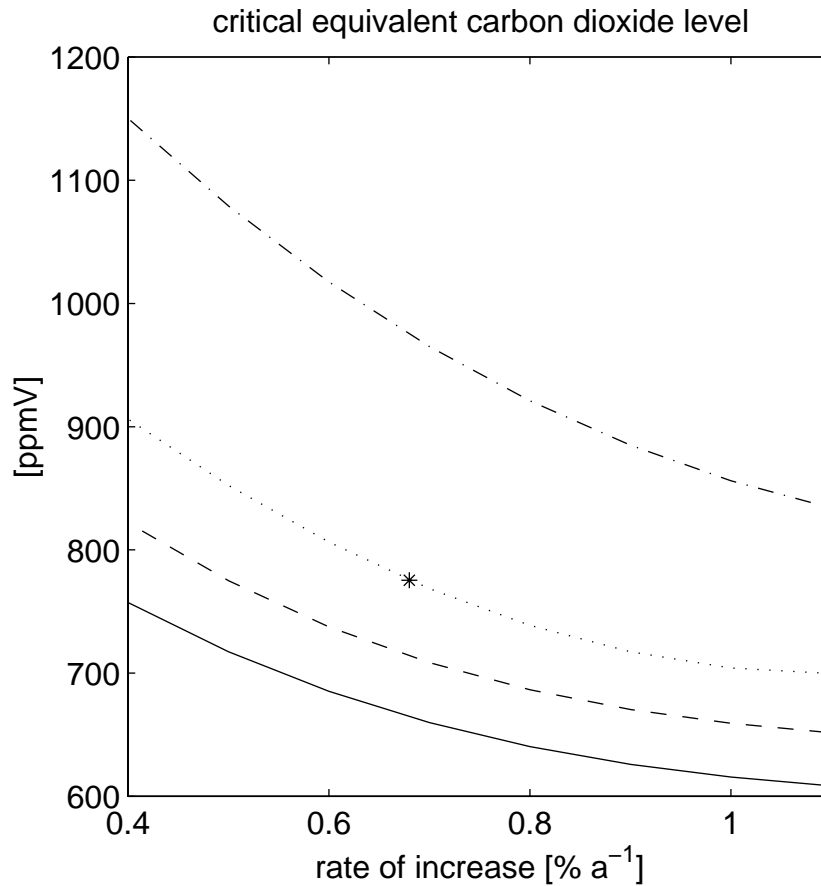
FIGURE 1: Critical atmospheric P_{CO_2,e} concentrations as a function of the rate of P_{CO_2,e} increase plotted for different values of climate sensitivity. Shown are polynomial fits to the model results reported by Stocker and Schmittner [1997]. The lines represent climate sensitivities of 4 °C (full line), 3.75 °C (dashed line), 3.5 °C (dotted line), and 3 °C (dash-dotted line). The star represents the critical atmospheric P_{CO_2,e} level for the approximate present rate of P_{CO_2,e} increase in the DICE model and the adopted climate sensitivity of 3.5 °C.
