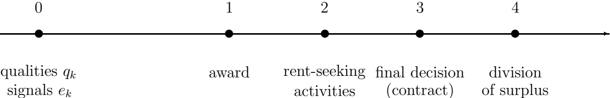
Figure 1: The timing of the games.
