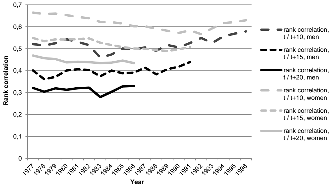
Figure 8: Rank correlation displaying long-term mobility for three different time horizons, by gender, 1977 - 1996
